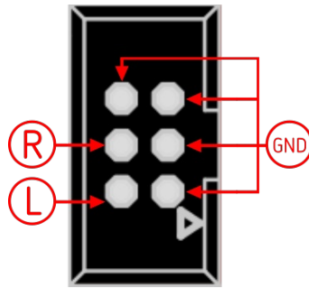
ST AMP Input Pinout
